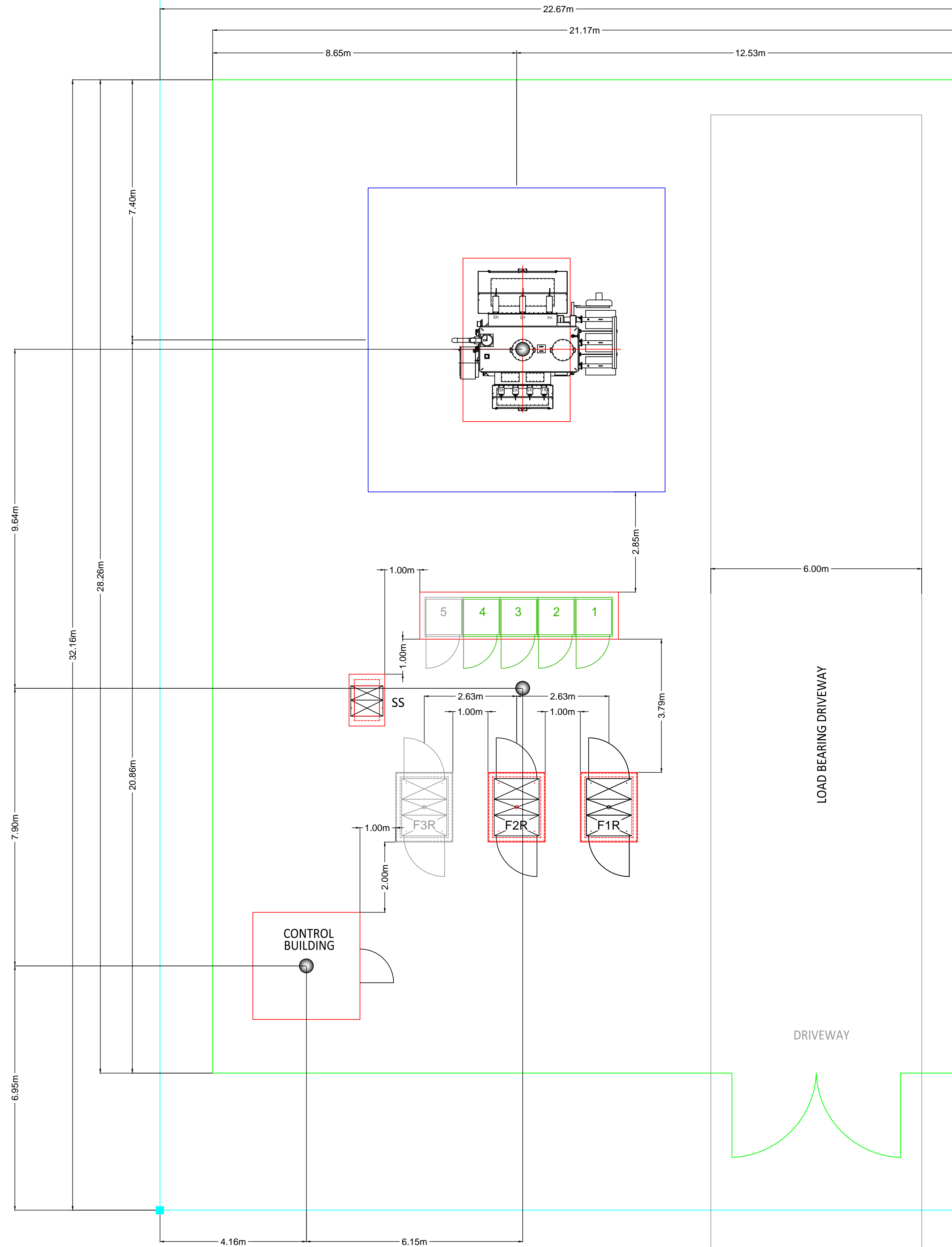
PROPOSED STATION LAYOUT SCALE - 1:75
