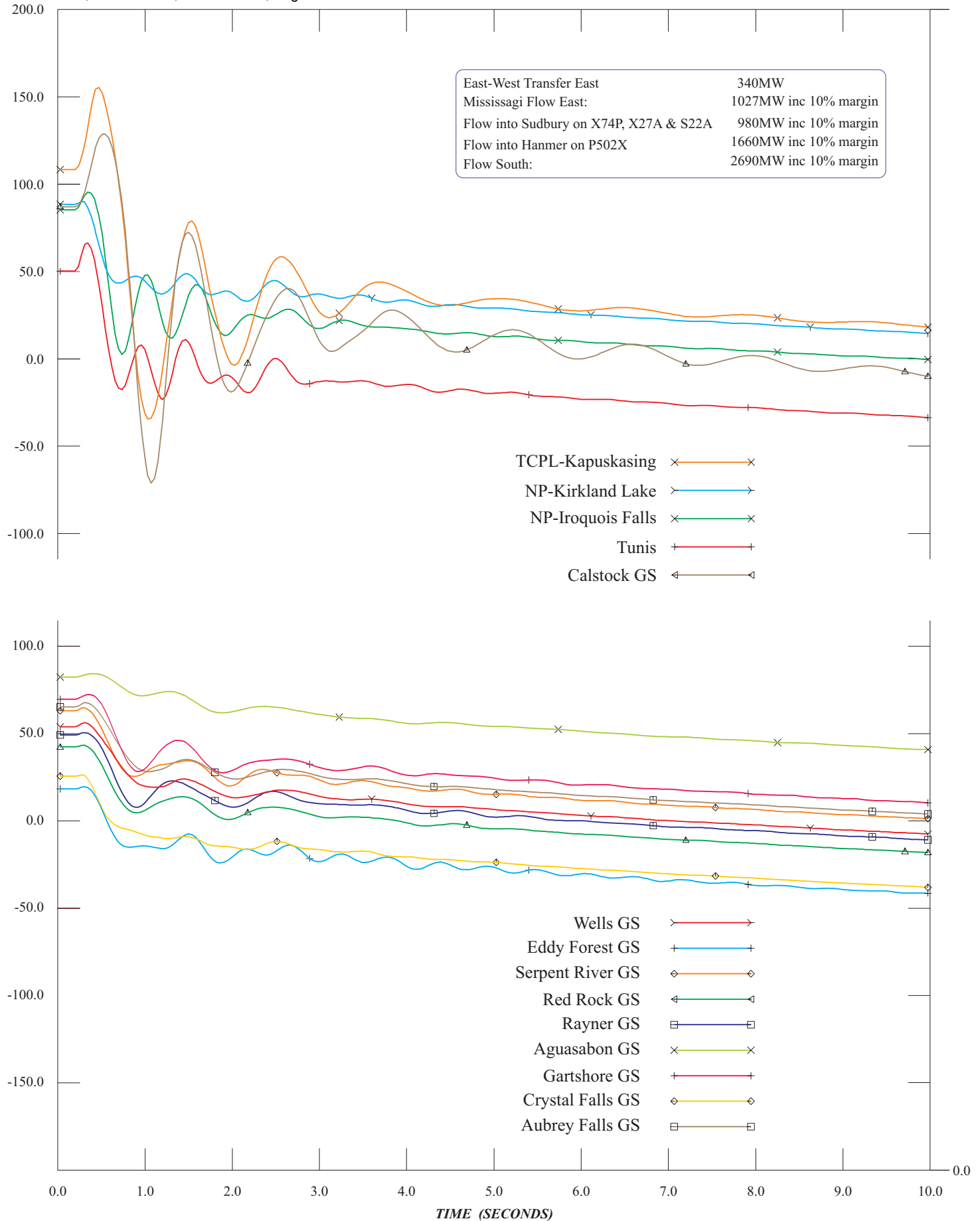
Generator Rotor Angle Responses to a 3-Phase fault on circuit D501P at Porcupine TS
