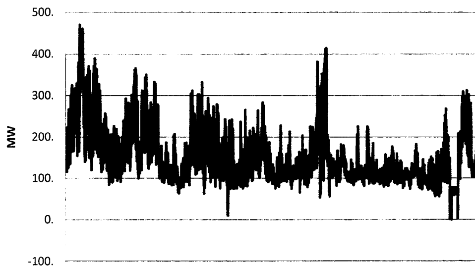
Figure 4: MW flow on N2M at Nanticoke SS
