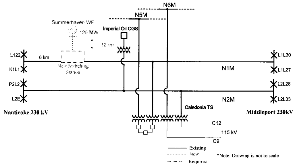
Figure 1: Summerhaven WF Connection to HONI Transmission System
