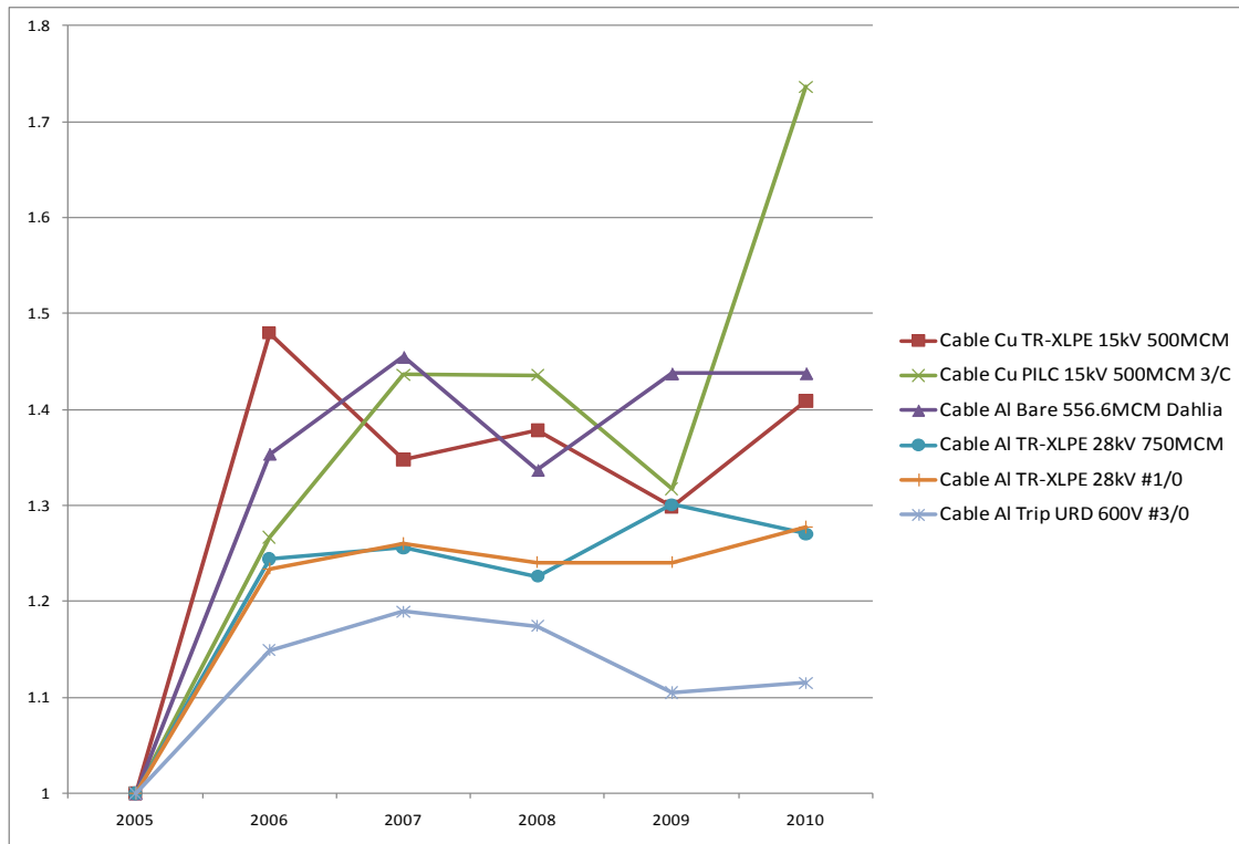
Figure 2 – Cable Costs Relative to 2005 Costs
