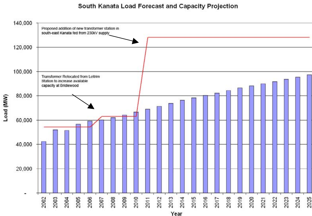
Figure 3 – South Kanata Load Forecast and Capacity Projection 2
