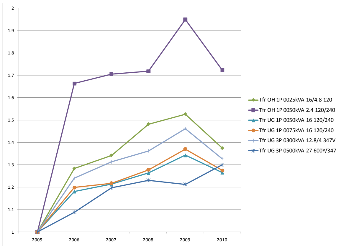
Figure 3 – Distribution Transformer Costs Relative to 2005 Costs
