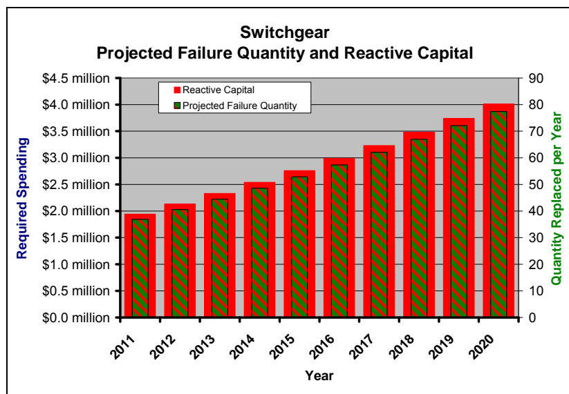
2 3 Figure 77. Distribution switchgear projected failure quantity and reactive capital.
