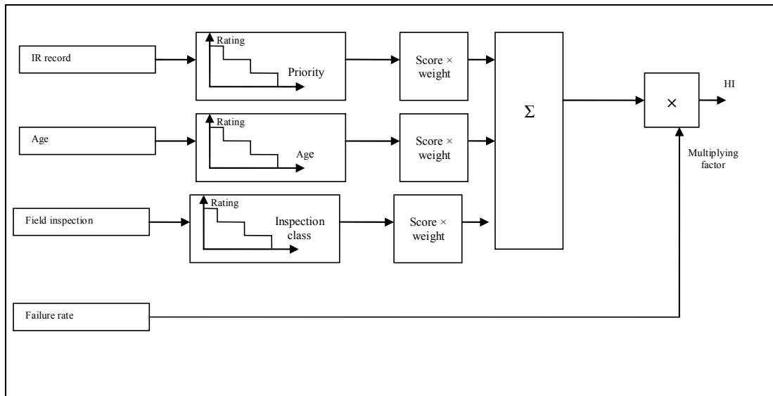
Figure 72. Distribution switchgear Health Index flowchart.
