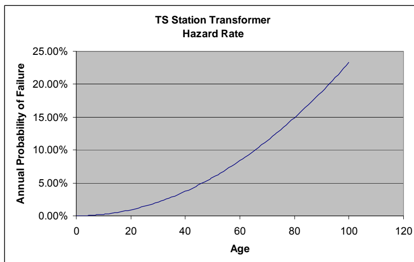
5 6 Figure 7. TS transformer hazard rate curve.
