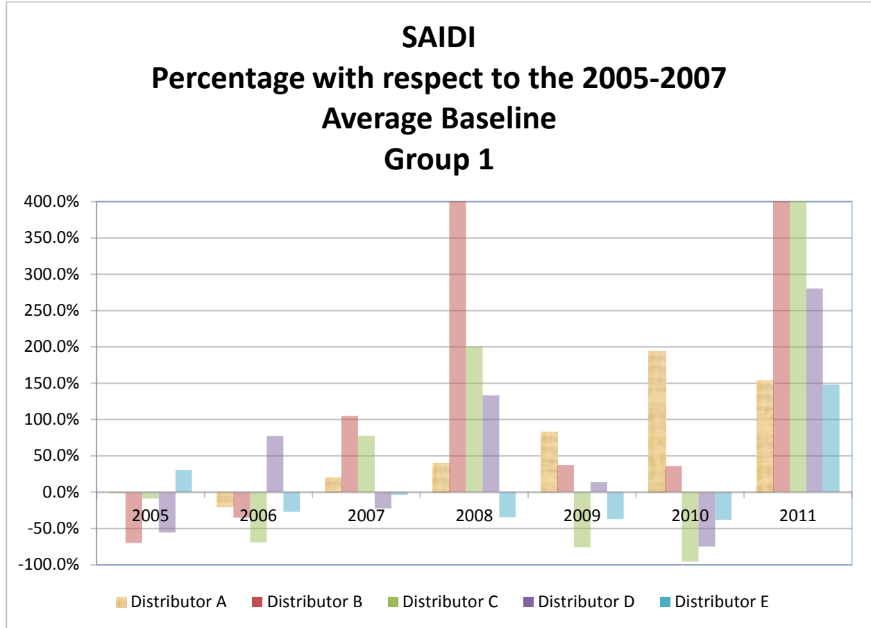
Exhibit 5.6. SAIDI Performance Relative to 2005-2007 Mean Select Small LDCs
