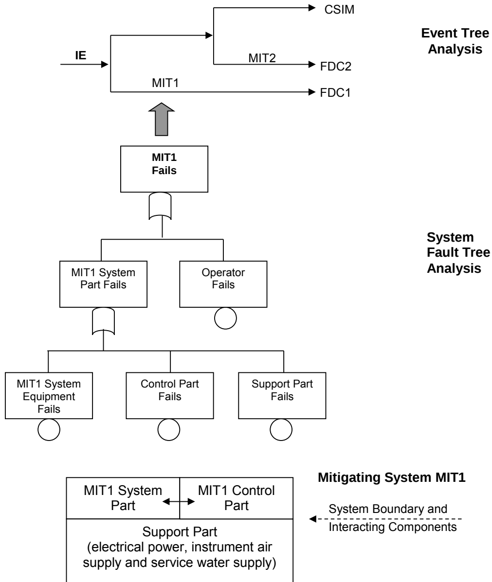
Figure 4: Fault Tree and Event Tree Integration
