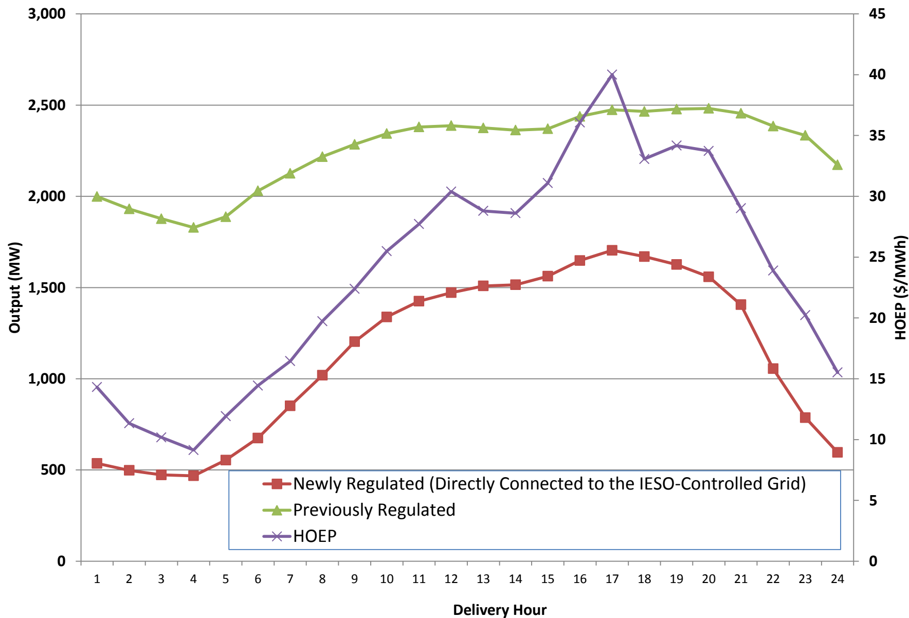
Figure 3: Hourly Hydro Output and HOEP (July to September 2013)
