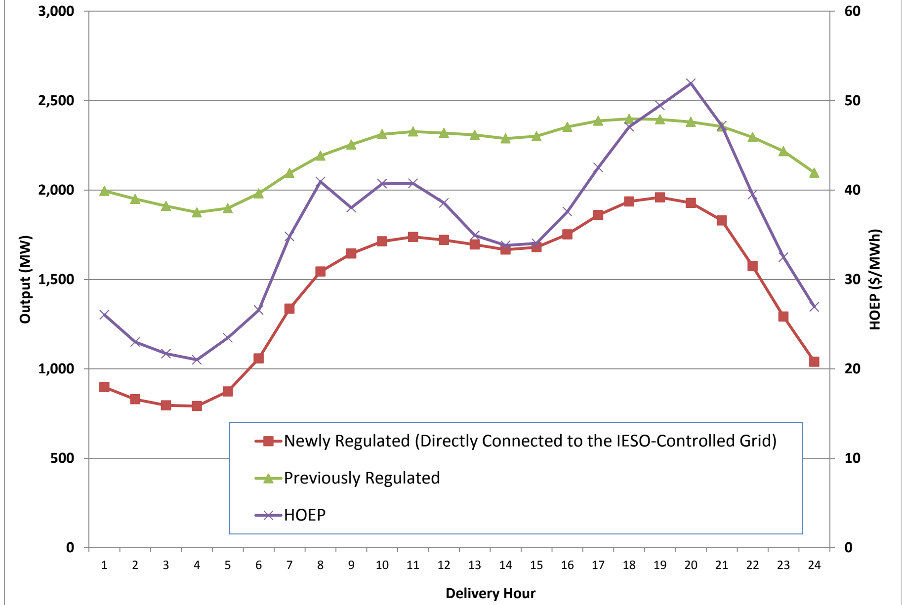
Figure 5: Hourly Hydro Output and HOEP (April 2013 to March 2014)
