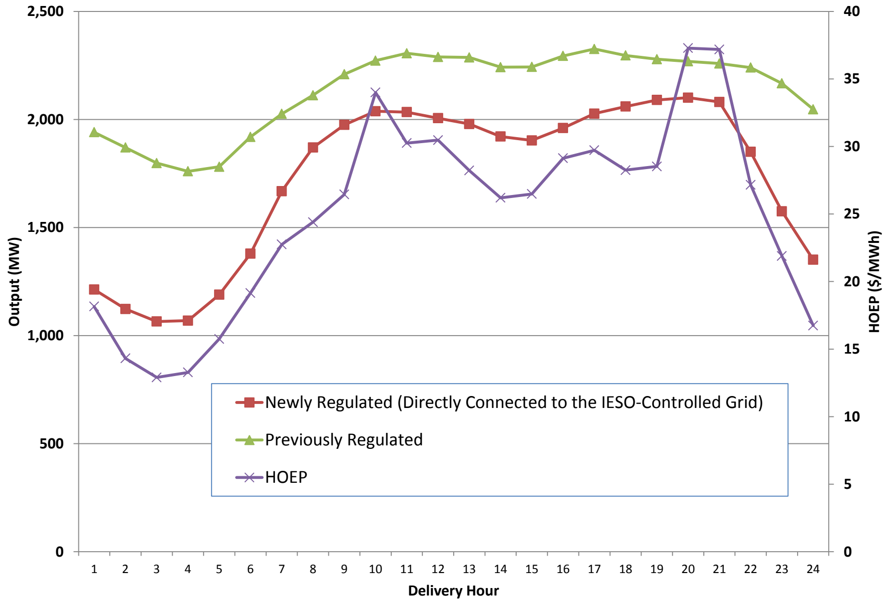
Figure 4: Hourly Hydro Output and HOEP (April to June 2013)
