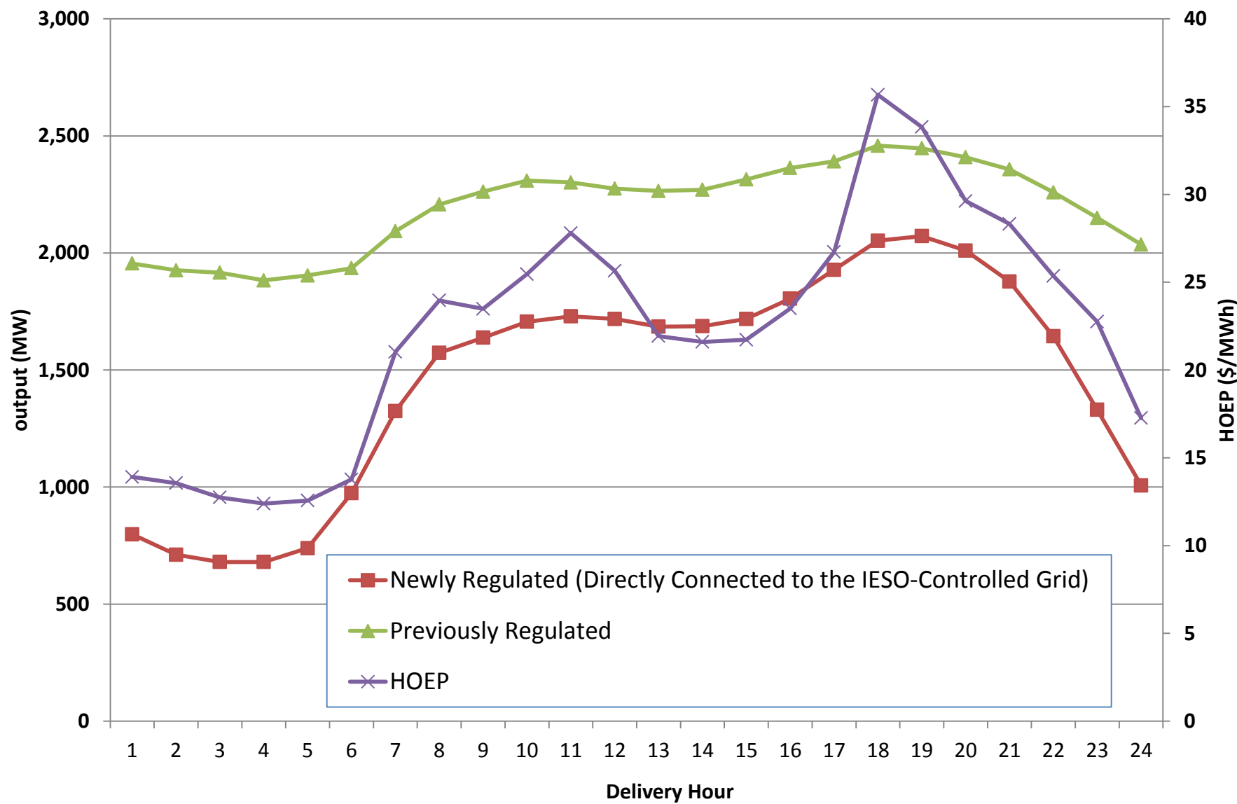
Figure 2: Hourly Hydro Output and HOEP (October to December 2013)
