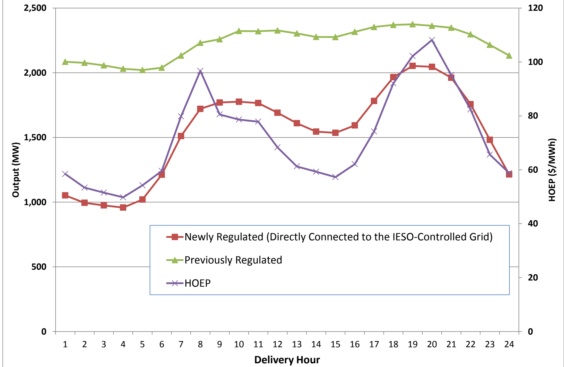
Figure 1: Hourly Hydro Output and HOEP (January to March 2014)
