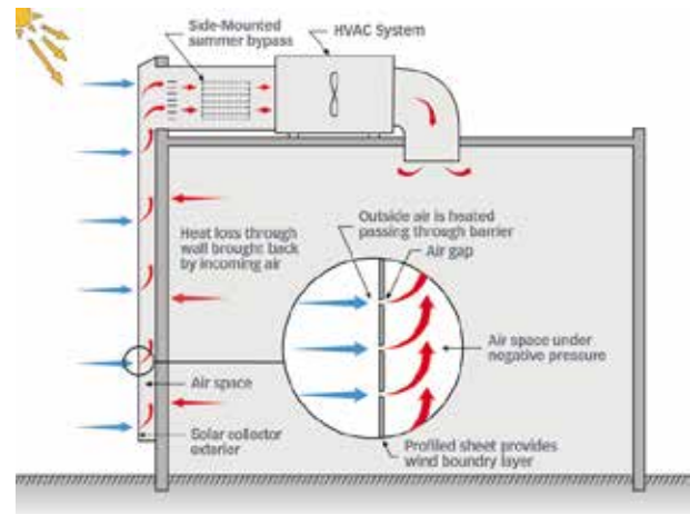
Solar thermal air system
