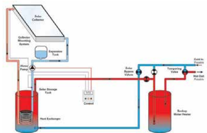
Solar thermal hot water system (Source: www.homepower.com [2])
