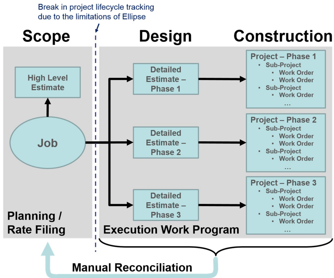
Figure 1: Project Lifecycle
