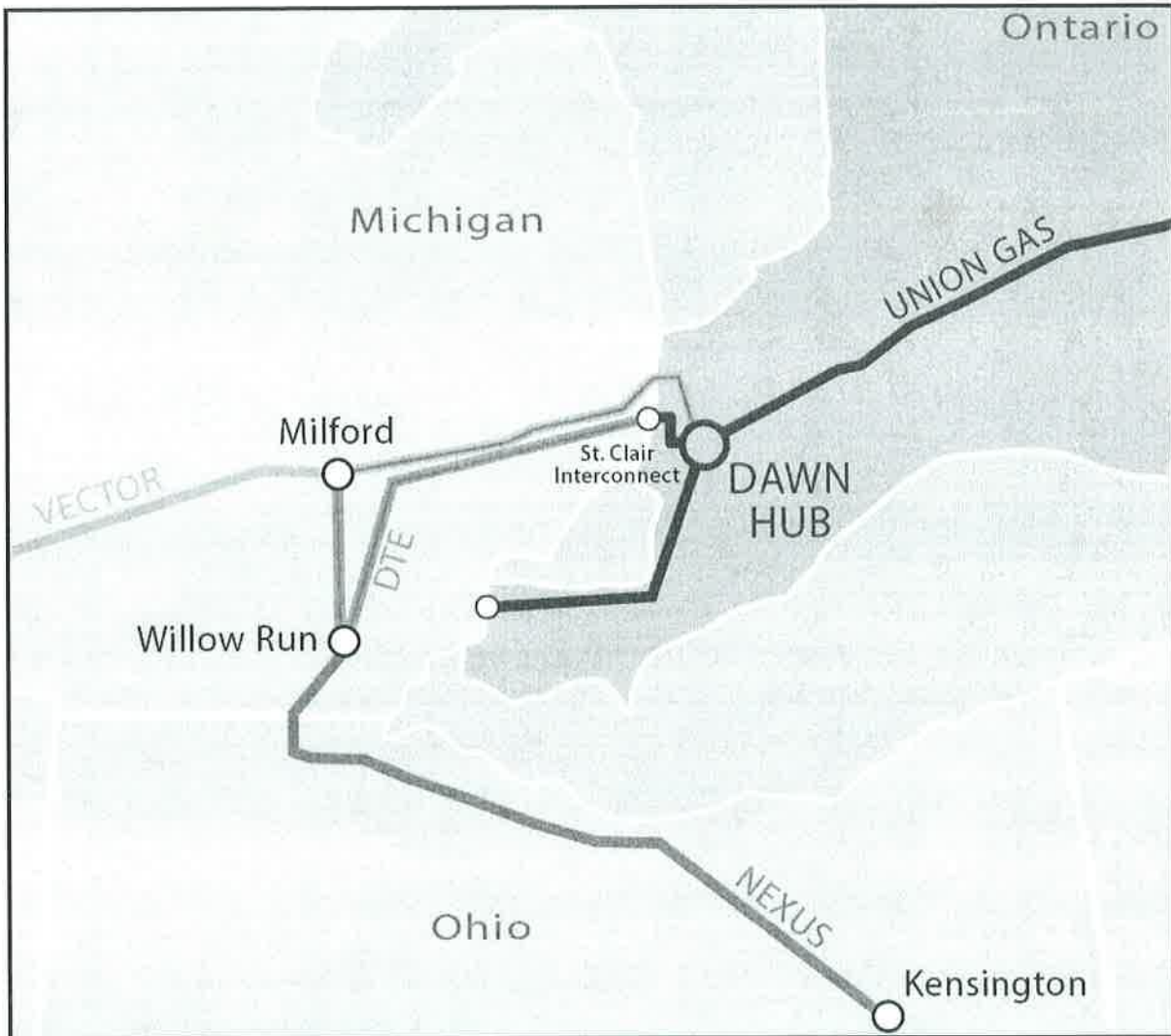
Figure 3-2 NEXUS Pipeline Paths to Ontario/Dawn
