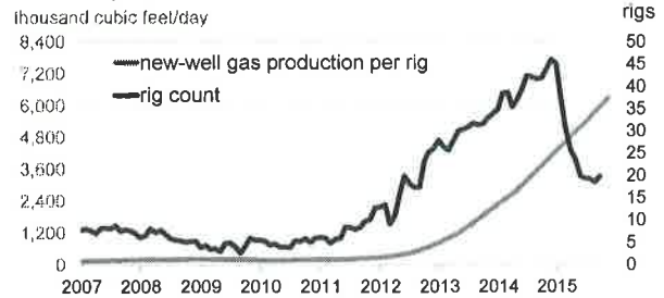
Utica Region New-well gas production per rig
