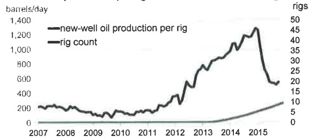
Utica Region New-well oil production per rig
