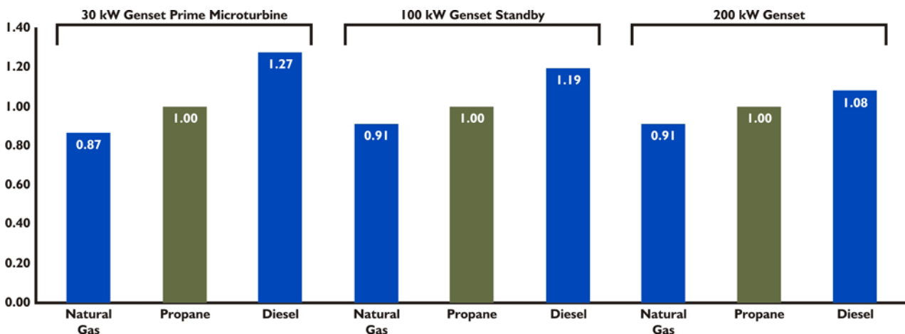
Figure 4.9. Distributed Generation
