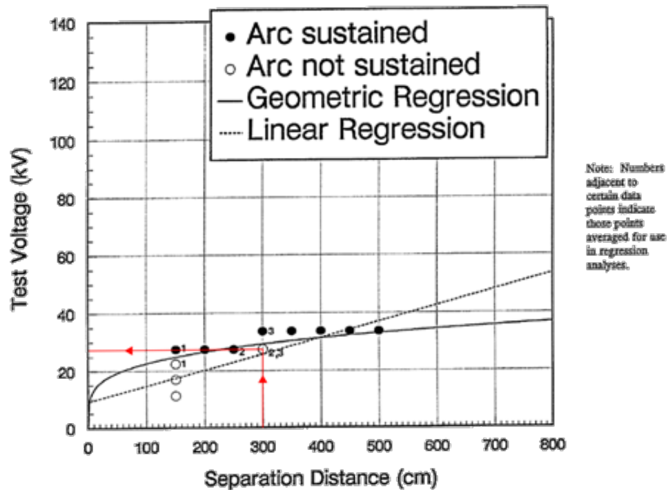
Figure 6-7. CEA Test Data in Top Soil (4 kA)
