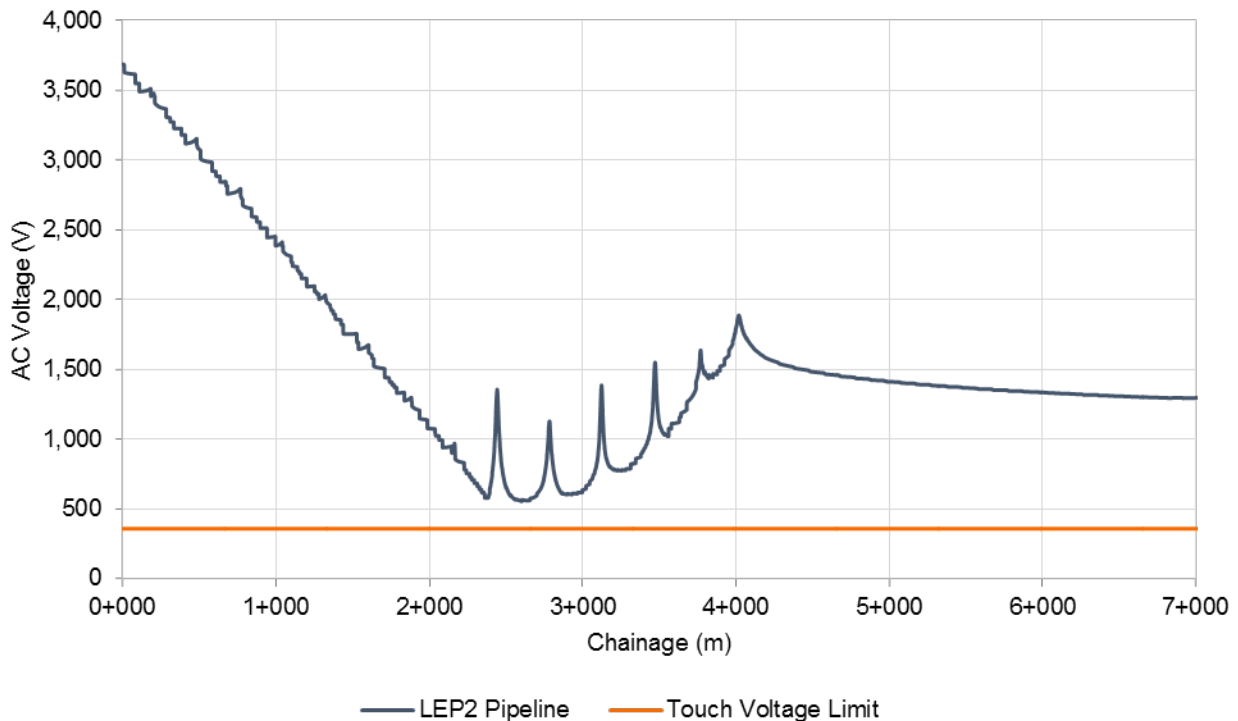
Figure 6-3. Predicted Unmitigated Touch Voltages under Fault Conditions
