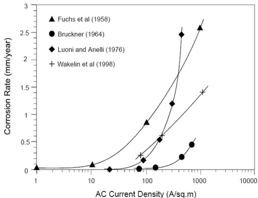
Figure 5-1. Corrosion Rate vs AC Current Density
