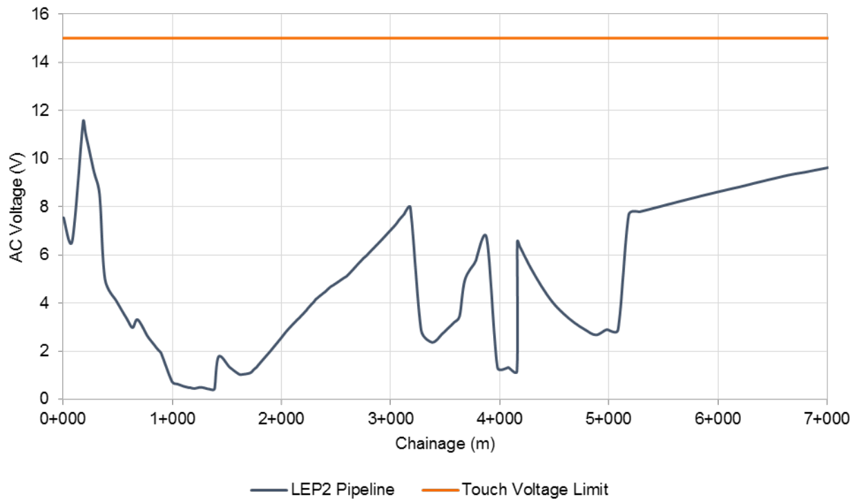
Figure 7-1. Predicted Mitigated Touch Voltages under Steady-State Conditions
