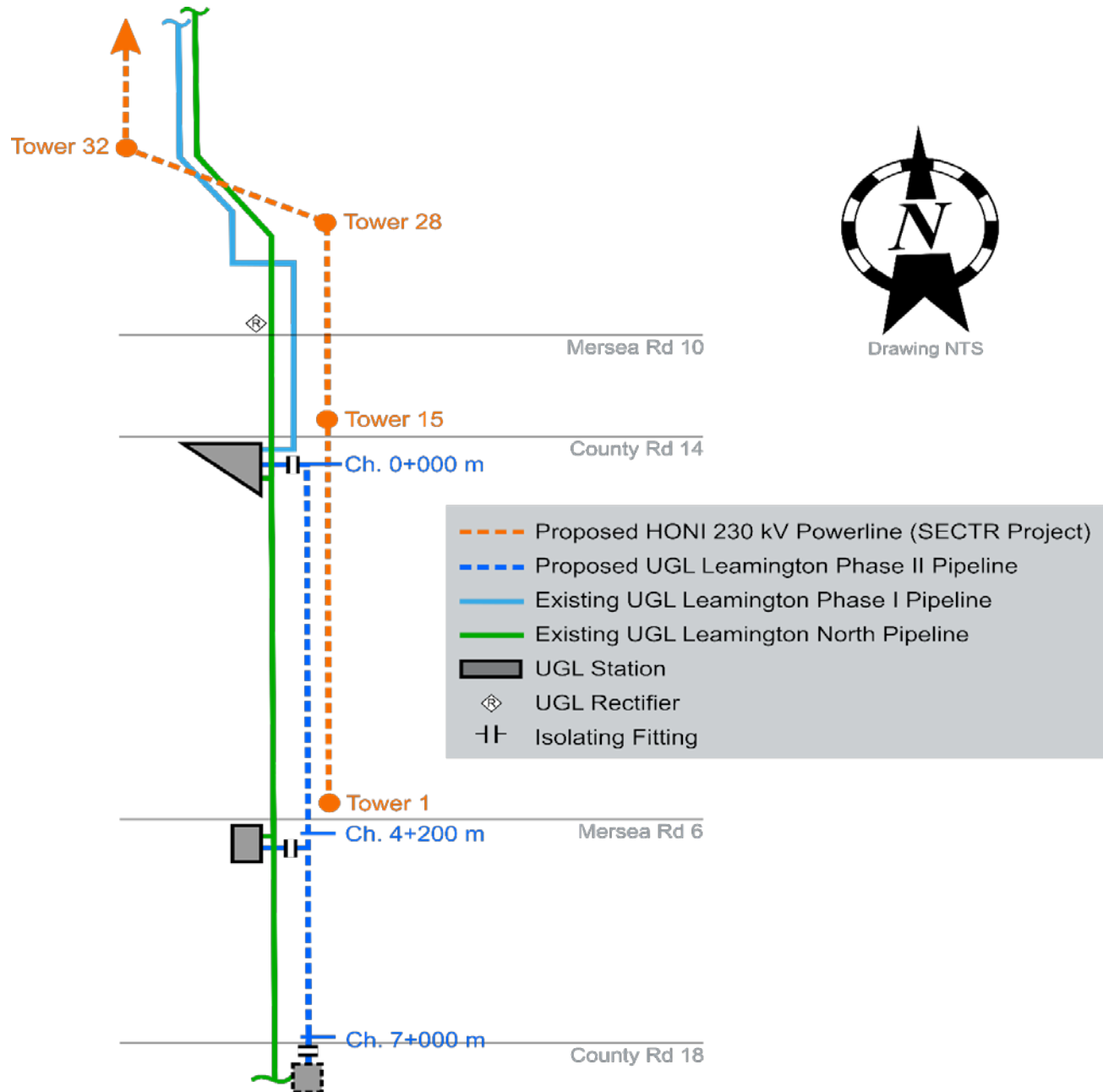
Figure 3-1. Pipeline/Powerline Right-of-Way Configuration
