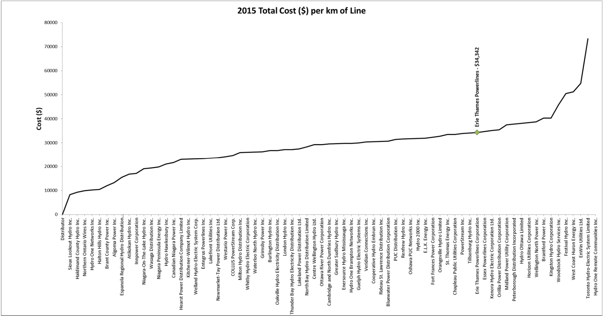
Figure 8: Total Cost ($) per km of Line
