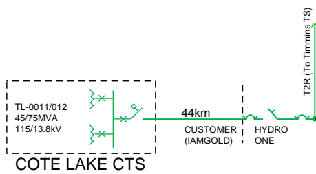
T2R / Iamgold Connection SLD
