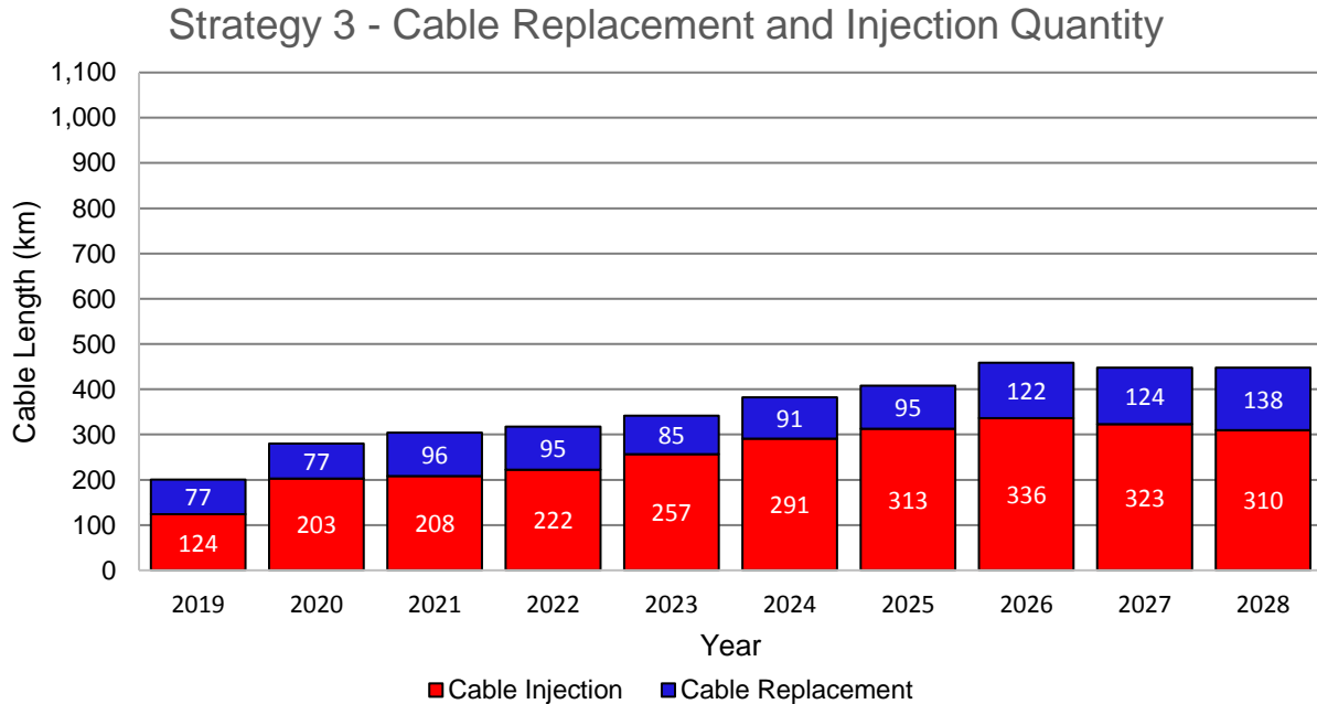
1 Figure A10 - 13: Cables Identified for Injection or Replacement under Strategy 3 (km)
