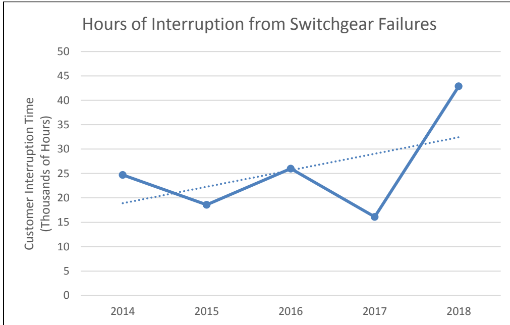
Figure 5.3.3 - 10: Customer Hours of Interruption from Switchgear Failures (2014-2018)
