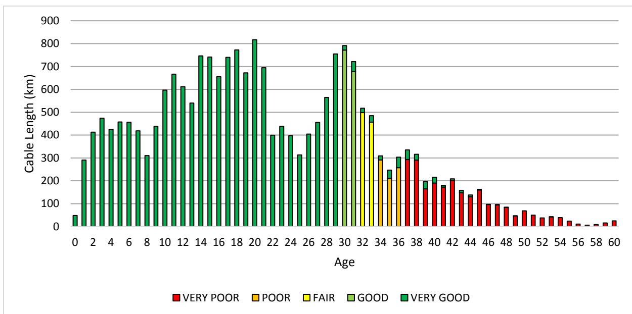
Figure A10 - 7: XLPE Cable by Condition
