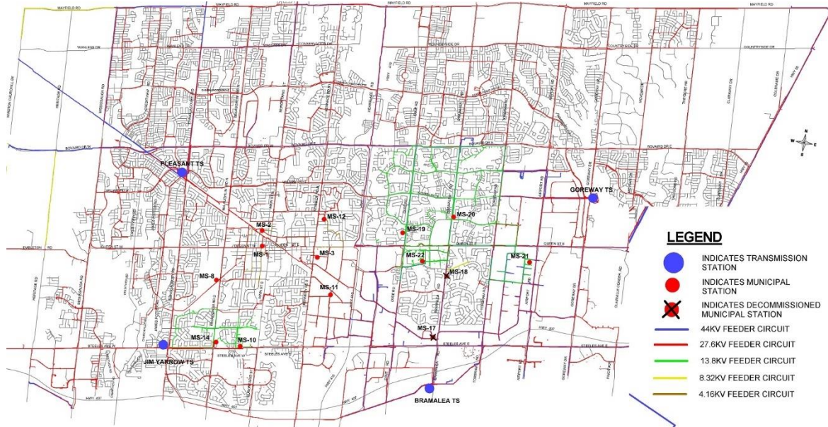
Figure A05 - 15: Low Voltage System - Brampton
