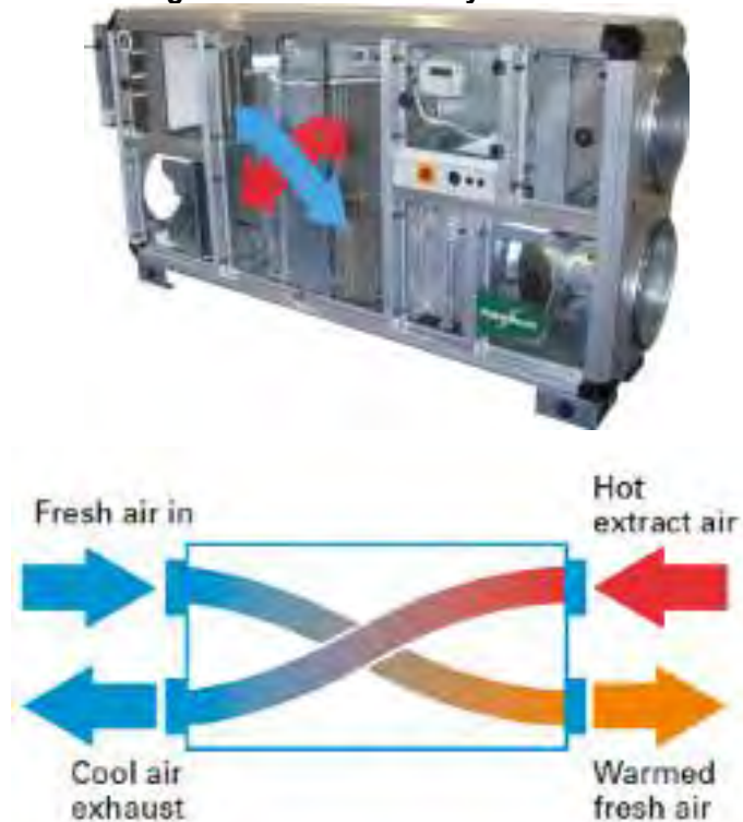
Figure 1: Heat Recovery Ventilator 3
