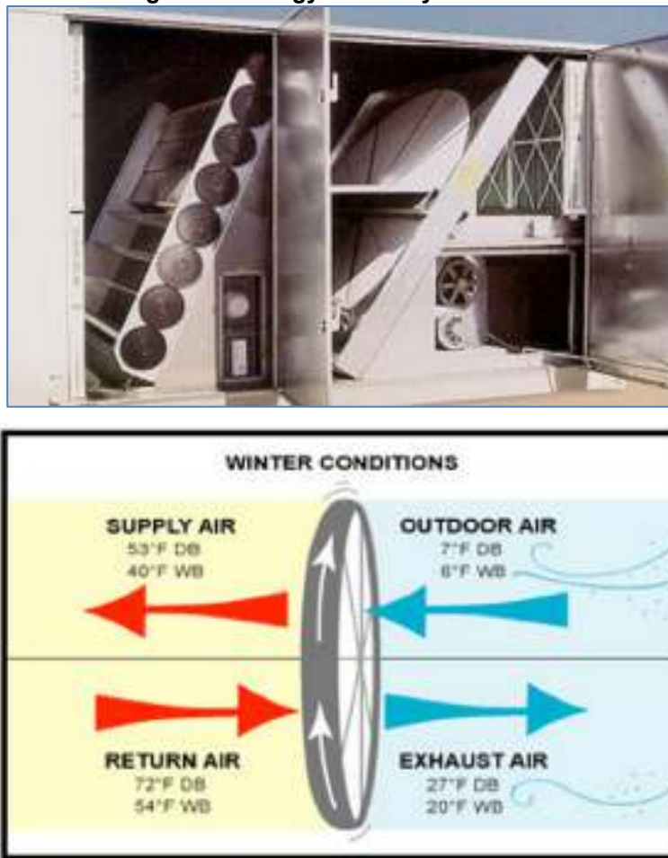
Figure 1: Energy Recovery Ventilator 4
