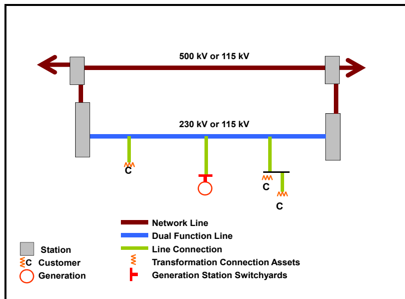
Figure 1: Transmission System Basic Elements
