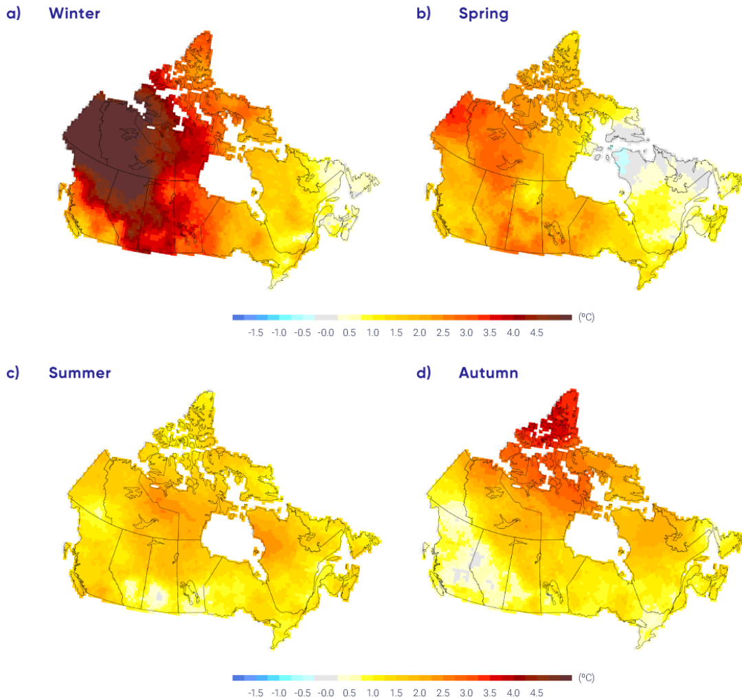
Figure 4.4: Trends in seasonal temperatures across Canada
