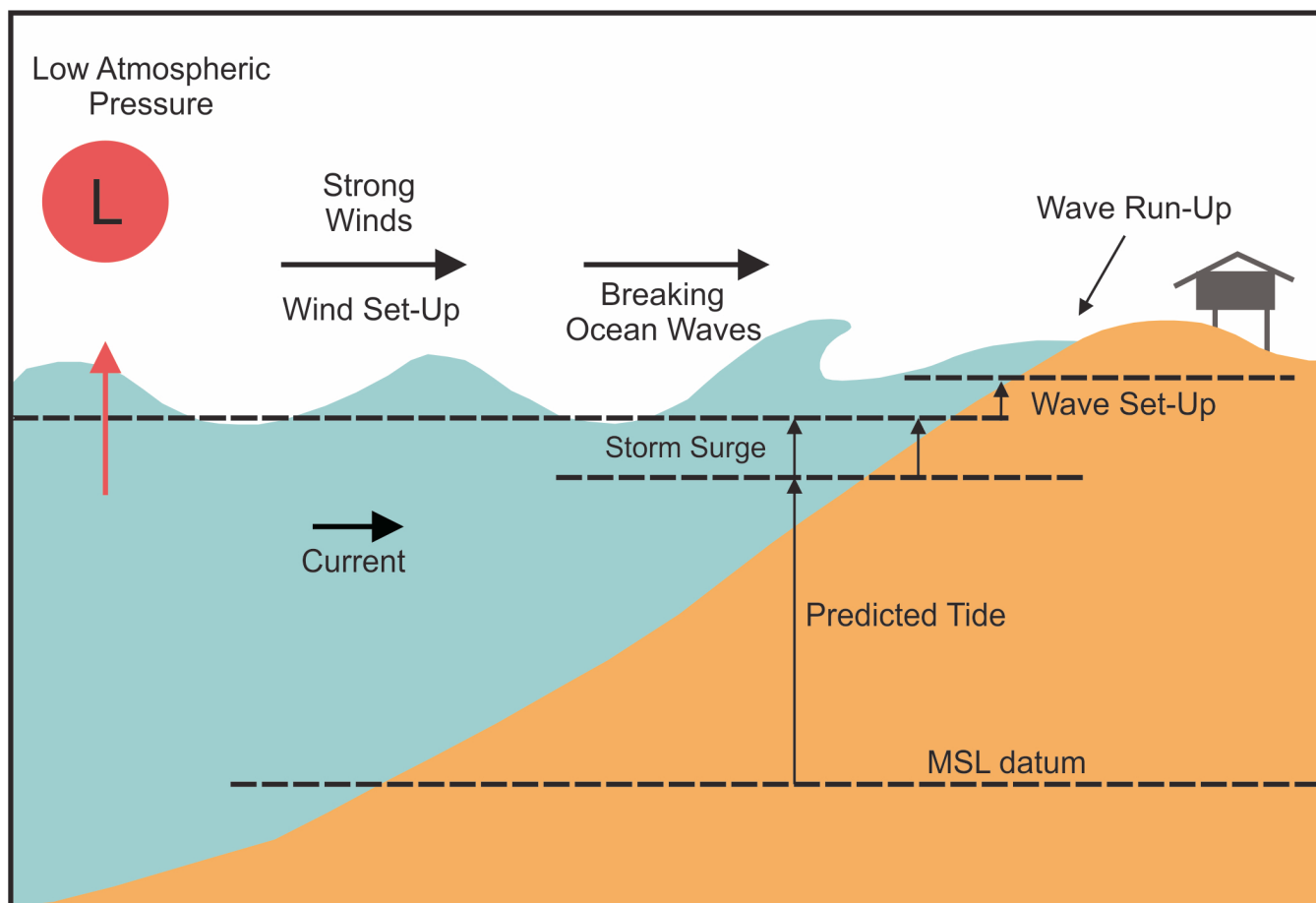
Figure 7.18: Factors contributing to storm surges
