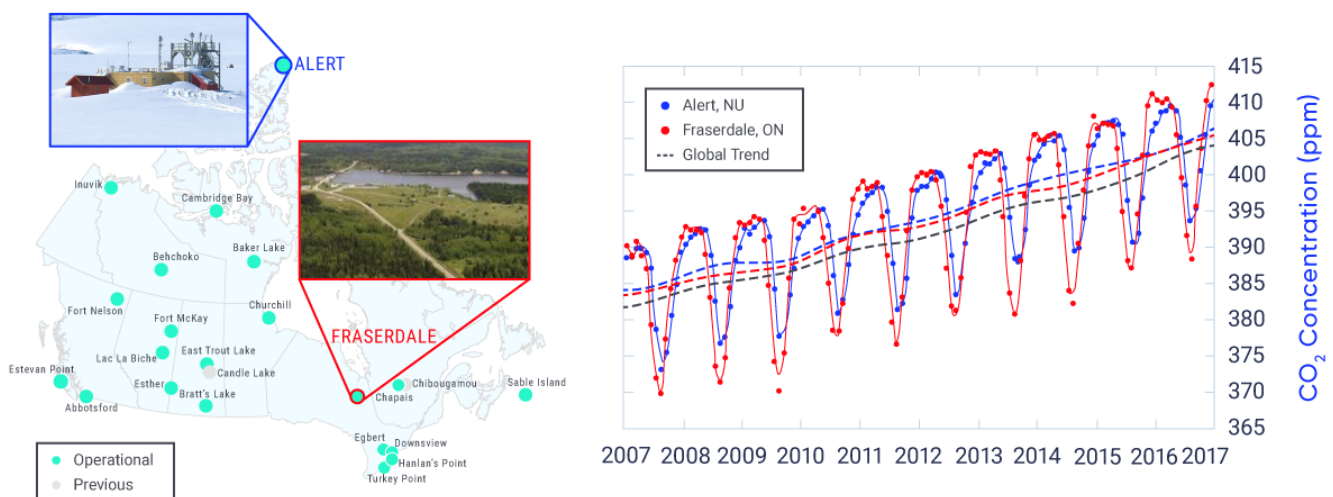
Figure 2.6: Canada's greenhouse gas monitoring network
