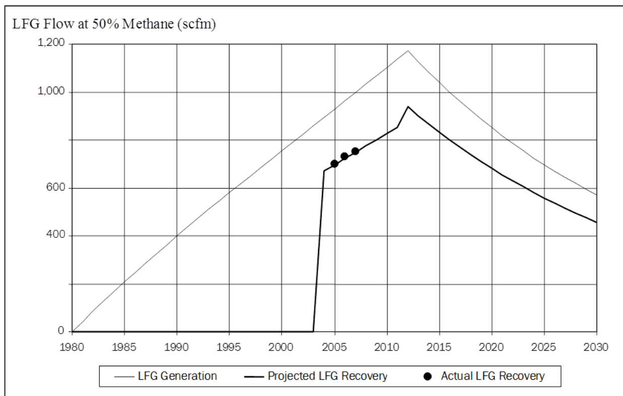
Figure 2-3. LFG Generation and Recovery Rates
