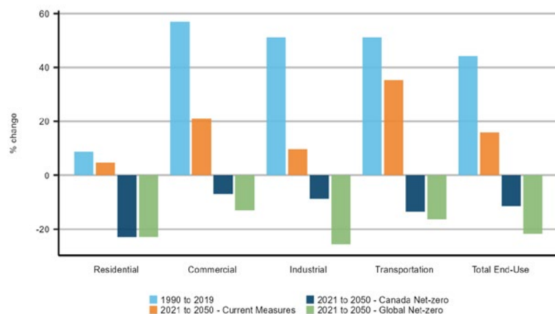
Figure R.5: Change in end-use energy demand by sector, 2021 to 2050, all scenarios
