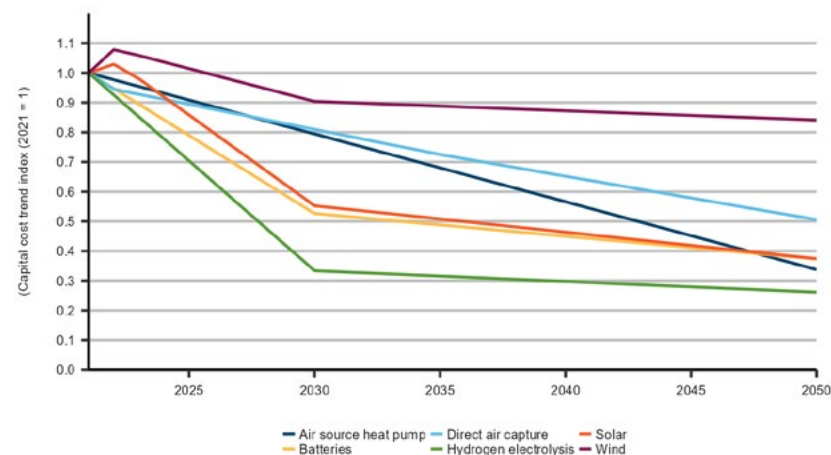
Capital cost trends for select technologies, Global Net-zero Scenario
