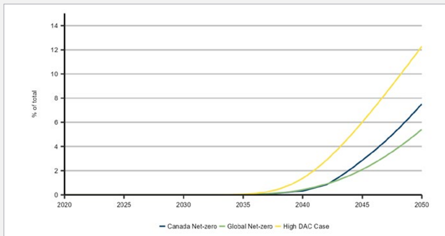
Figure R.45: Negative emissions from DAC, as a % of total GHG emissions in 2005, all scenarios
