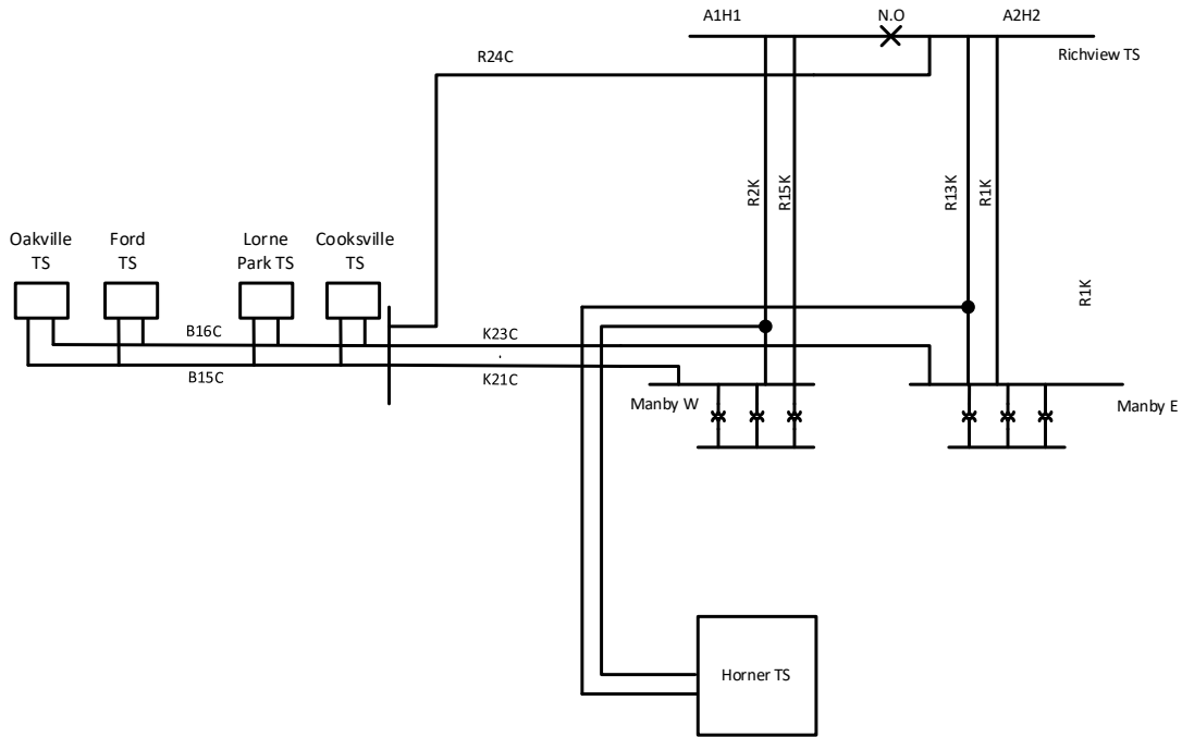
Figure 1- Richview TS x Manby TS Transmission – Existing facilities
