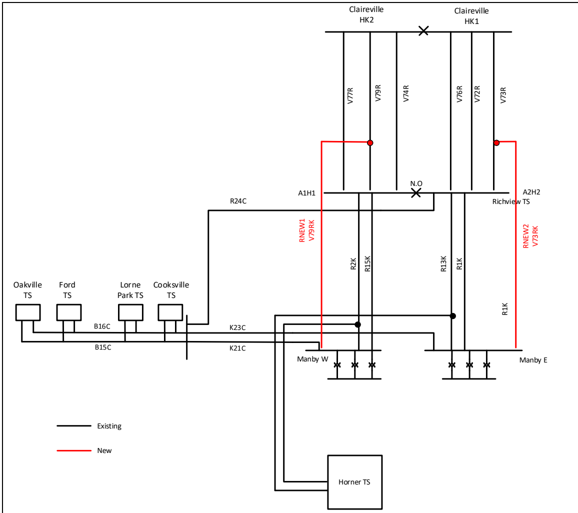
Figure 3- Richview TS x Manby TS Transmission – Stage 2 facilities
