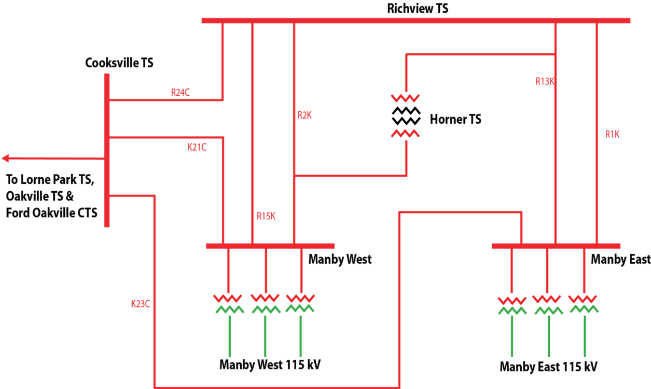
Figure 2 | Single Line Diagram of Richview South Area
