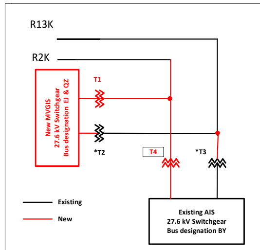
Figure 2- Horner TS: Proposed Facilities
