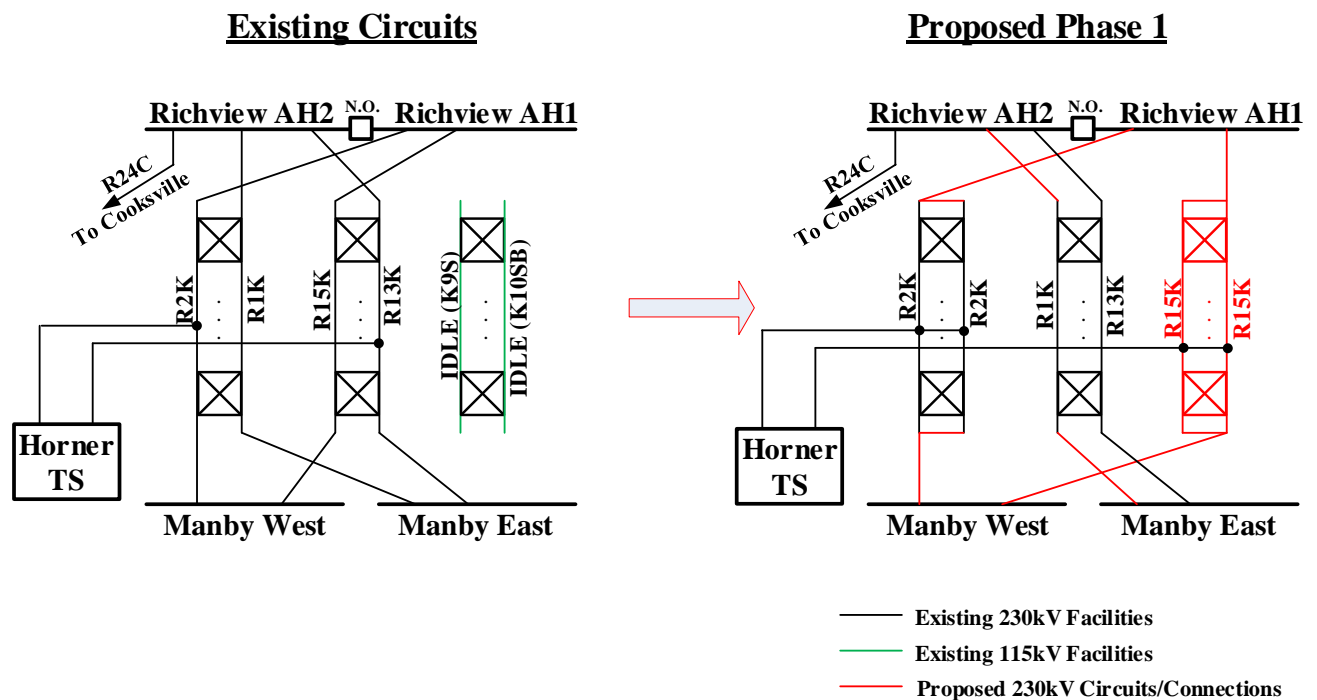
Figure 1: Existing and Proposed Phase 1 Transmission Circuits Between Manby TS and Richview TS
