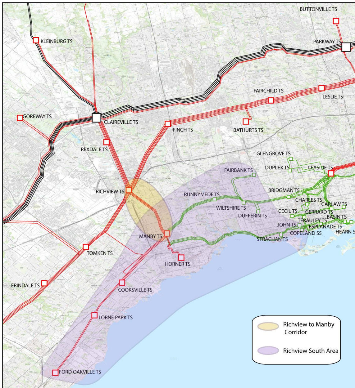
Figure 1 | Area Supplied by the Richview to Manby Corridor
