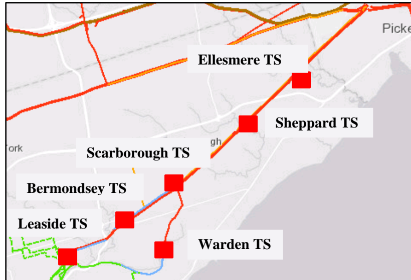
Figure 7-9: Bermondsey TS and Surrounding Stations
