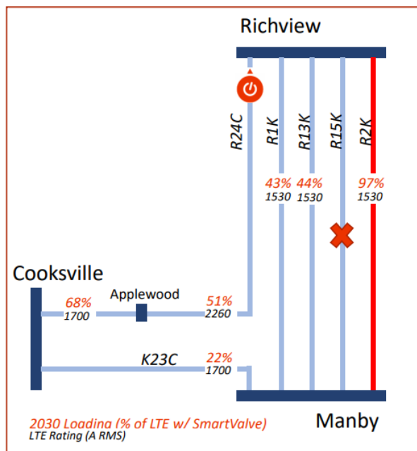
Figure 3 | Diagram showing most limiting contingency and element and proposed location of SSSC technology (Source: Smart Wires Inc.)
