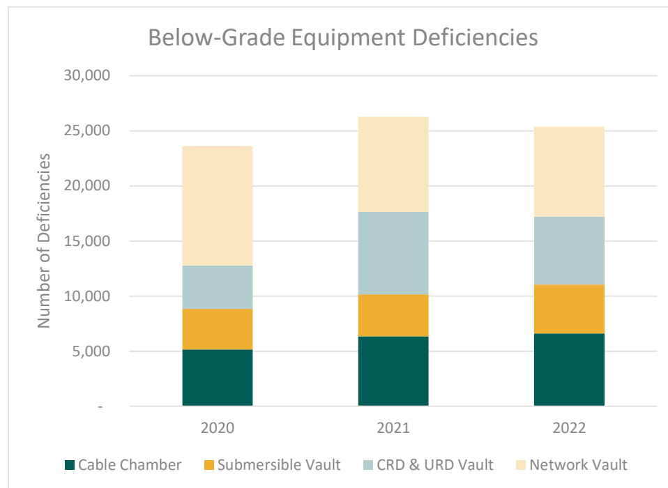
Figure 5: Below-Grade Equipment Deficiencies Identified Between 2020 and 2022
