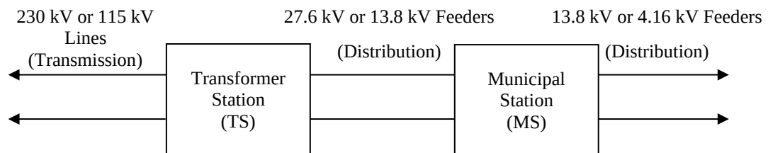
Figure 18: System Configuration
