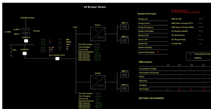
Figure 2: Energy Centre Display of a Battery Storage Site
