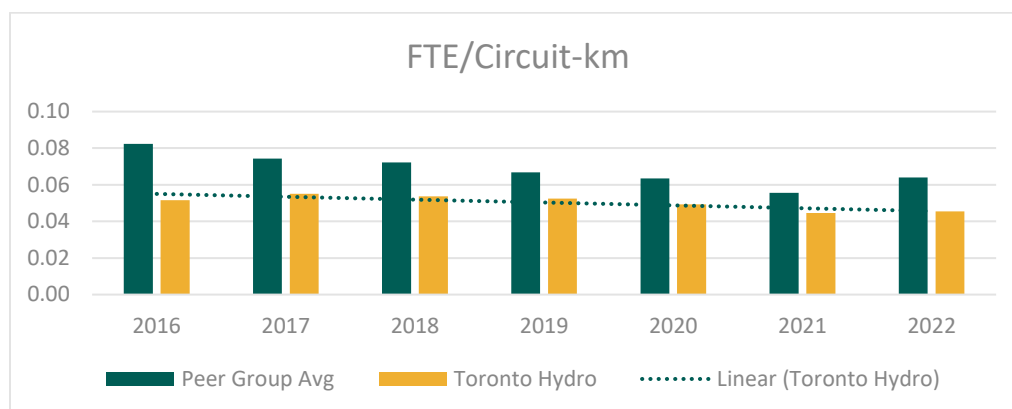
Figure 7: FTE per Circuit-Km
