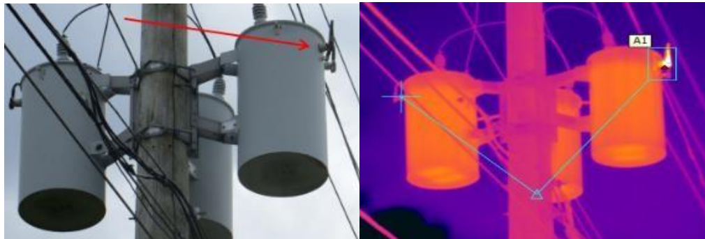
Figure 1: Secondary Connection on Pole-Mounted Transformer (Left) with an Infrared Thermography Image of the Same Asset Denoting a Hot Spot at A1 (Right)
