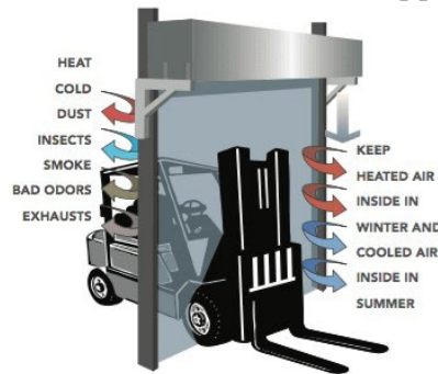
Figure 1. Air Curtain Installation 1
