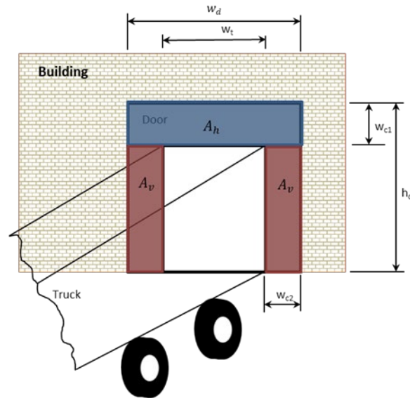
Figure 3 Dock Door opening area
