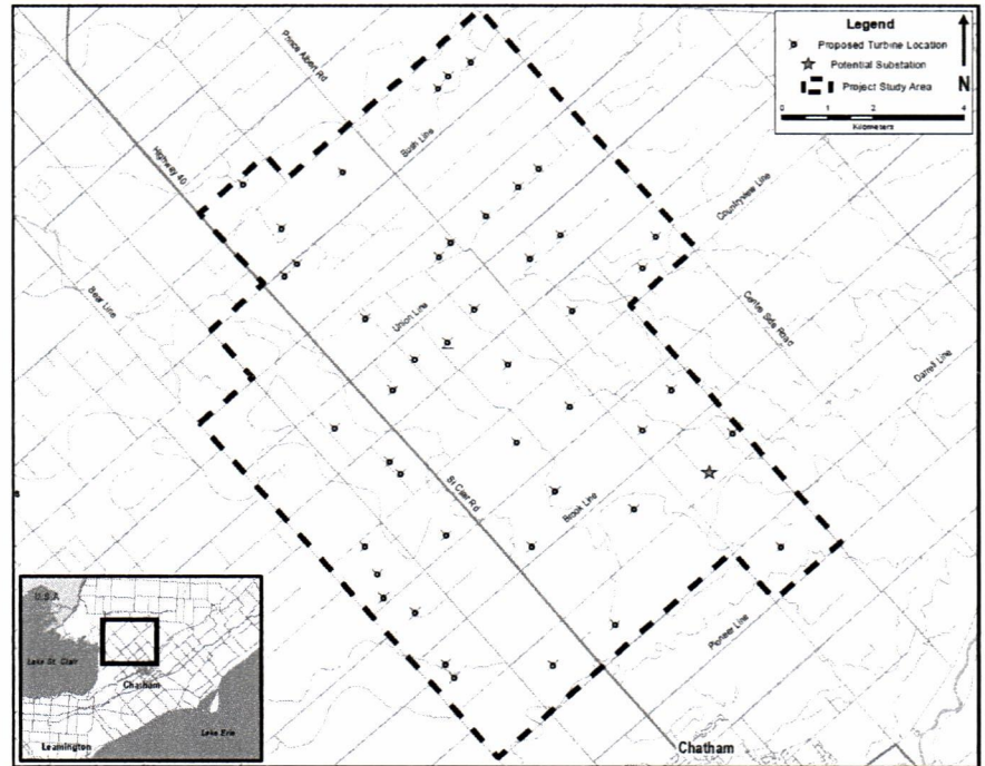
Location of Wind Turbines and Substation
