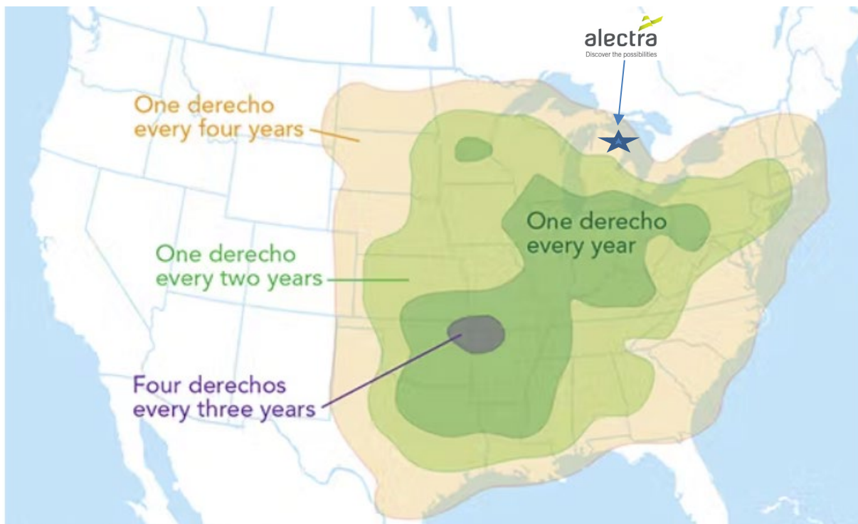
Figure 5.3.2 - 3 Derecho Event Occurrence Rate 64
