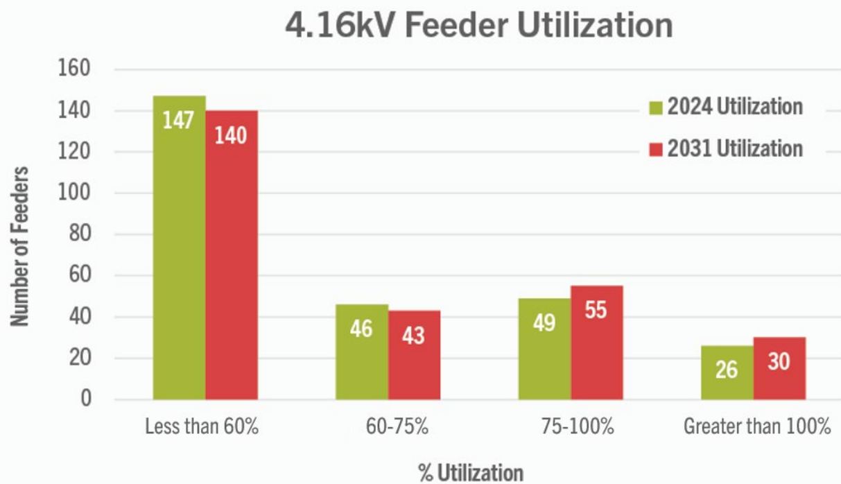
Figure 5.3.2 - 89 4.16kV Feeder Utilization
