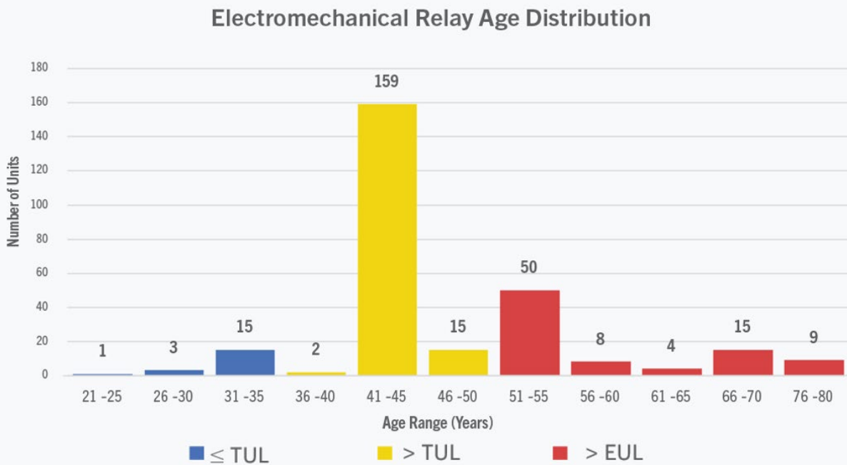
Figure 5.3.2 - 81 Electromechanical Relay Age Distribution
