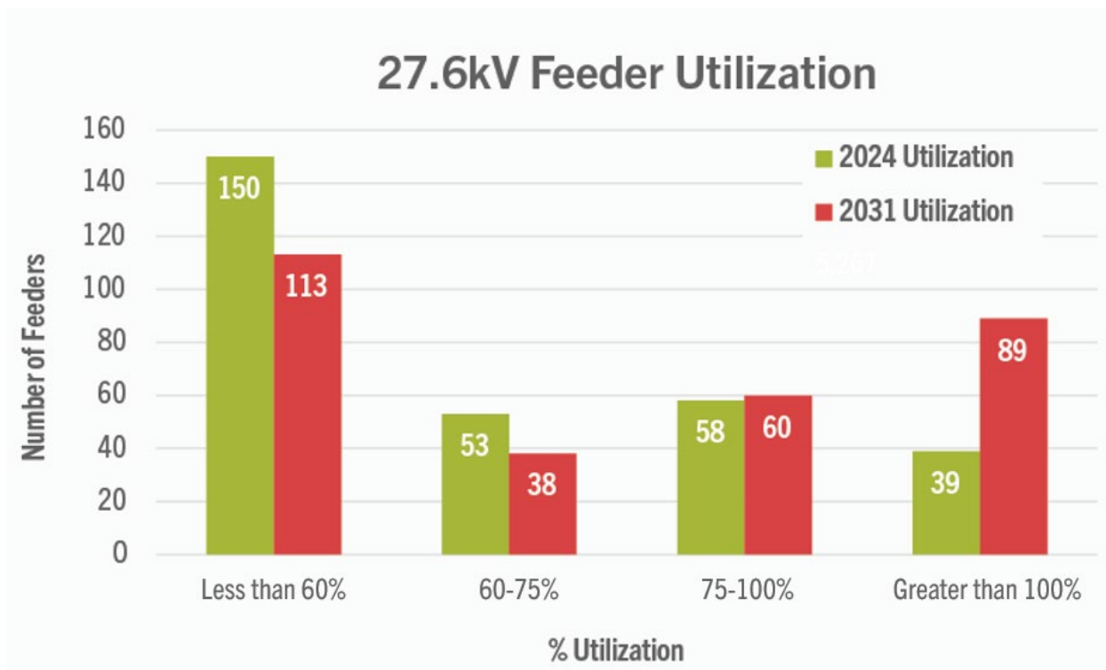
Figure 5.3.2 - 92 27.6kV Feeder Utilization
