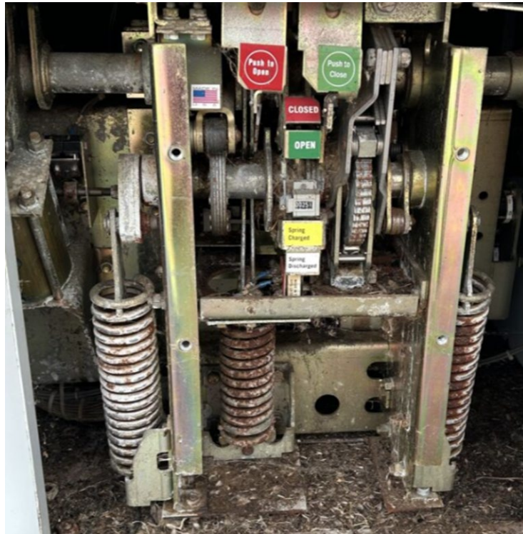
Figure 5.3.2 - 77 Interior of Rusting Outdoor Circuit Breaker
