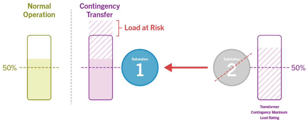
9 10 Figure 5.3.2 - 86 Contingency N-1 Criterion for Two Substation Network
