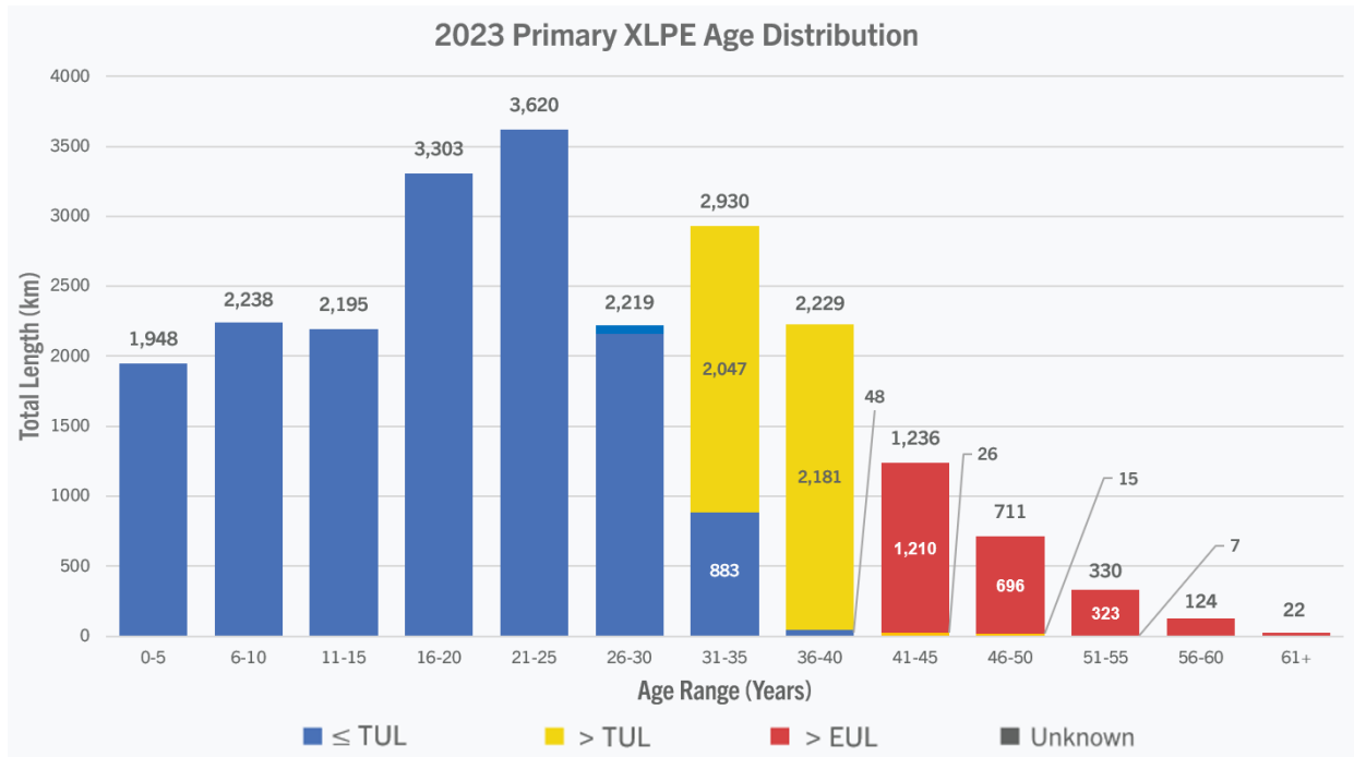
Figure 5.3.2 - 63 Primary XLPE Cables Age Distribution
