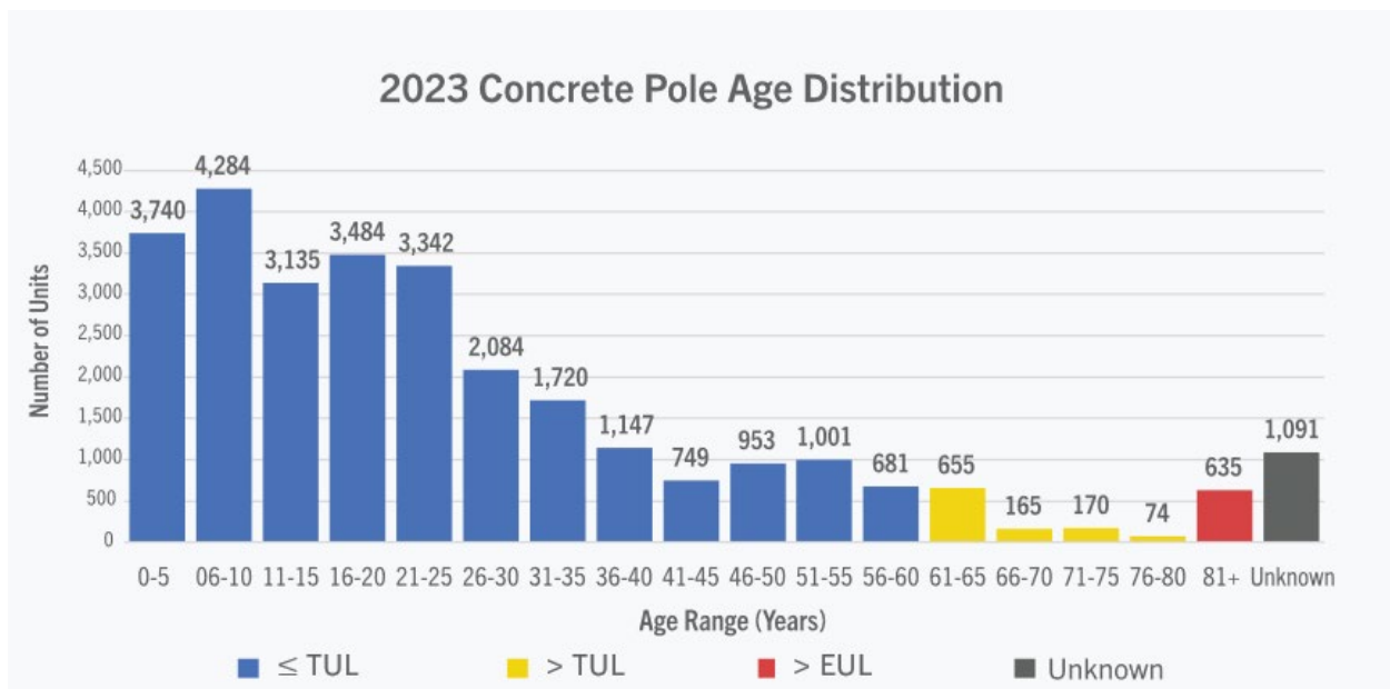
Figure 5.3.2 - 45 Concrete Pole Age Distribution
