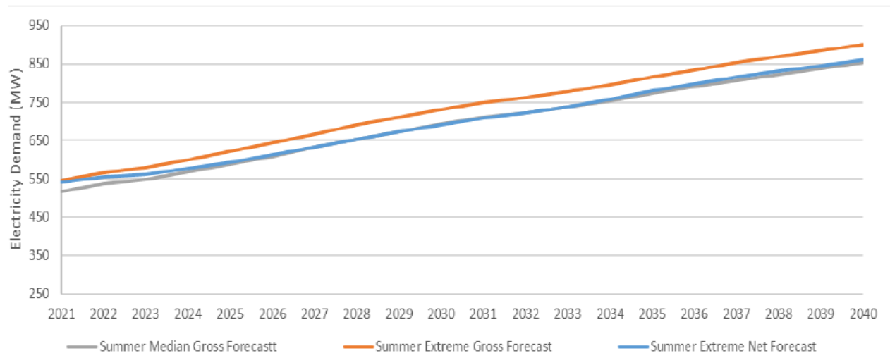
Figure 5.2.2 - 4 Barrie/Innisfil Demand Forecast Scenarios 24
