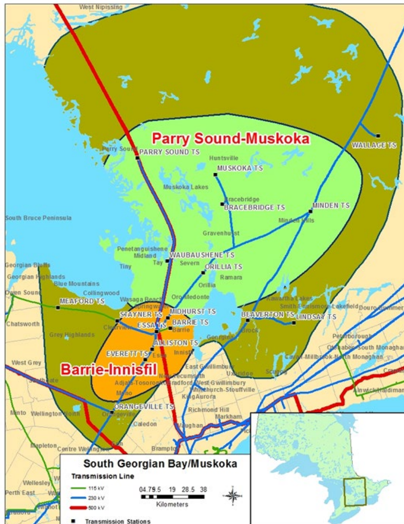
Figure 5.2.2 - 5 Parry Sound/Muskoka Transmission System 25
