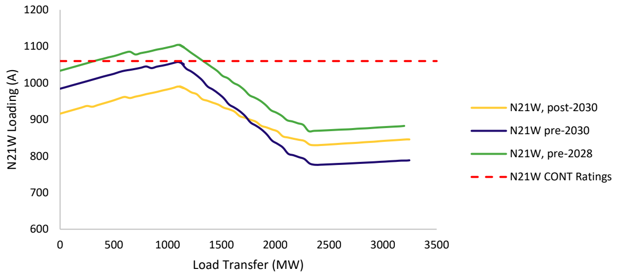
Figure 10 | Sensitivities to N21W Pre-contingency Loading without Reinforcements
