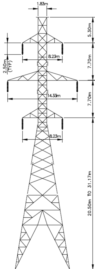
Figure 1: 230kV Double-Circuit Suspension Tower Structure (Type: X10S-R)
