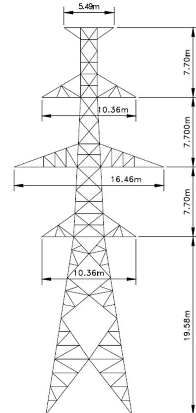
Figure 3: 230kV Double-Circuit Medium Anchor Tower Structure (Type: X10M-R)
