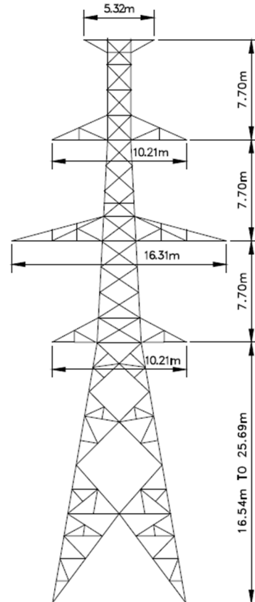
Figure 2: 230kV Double-Circuit Heavy Anchor Tower Structure (Type: X10H-R)
