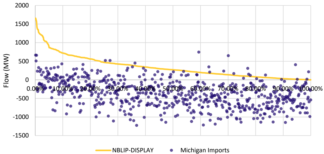
Figure 12 | Historical NBLIP Duration Curve with Michigan Imports, 2018-2022
